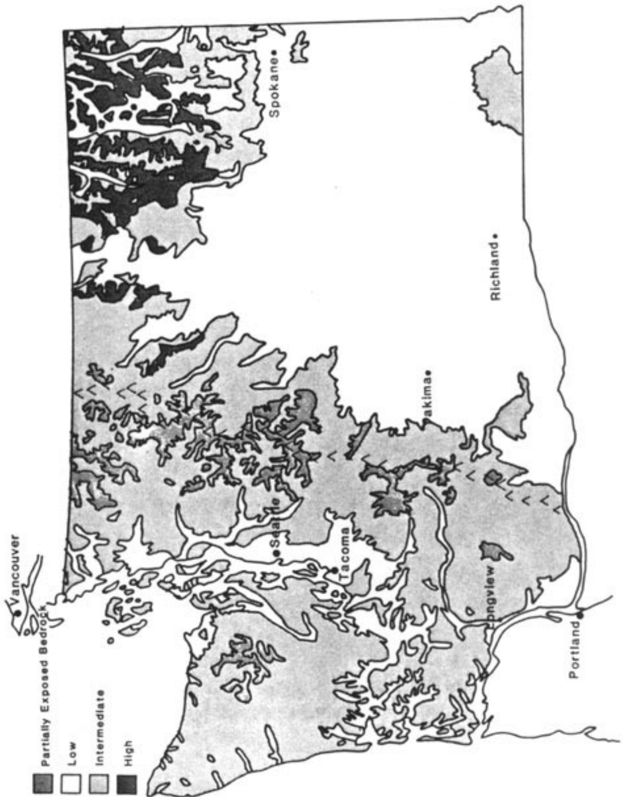
Figure 2. Relative sensitivity of Washington soils to release of cations to aquatic resources with acid deposition.
